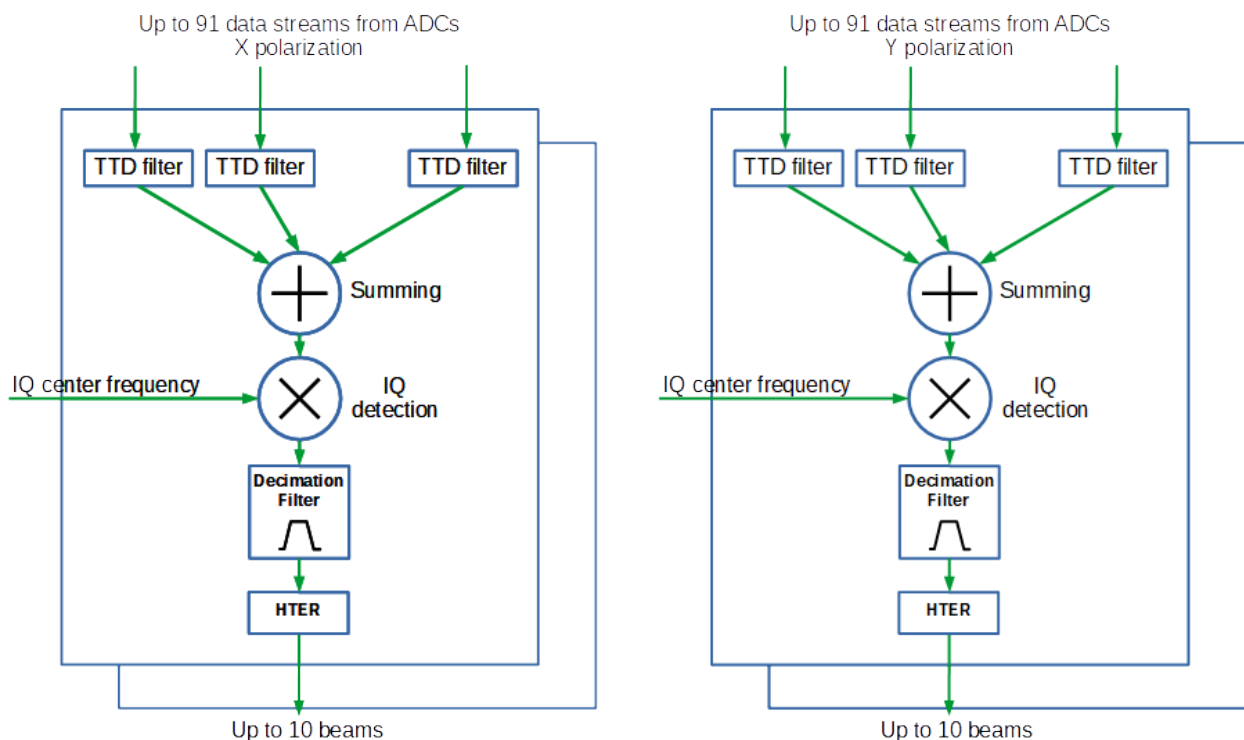
Diagram 2. Beamformer functions.
