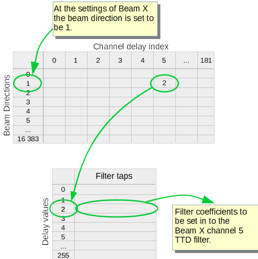
Diagram 3. Beam directions mapping..
