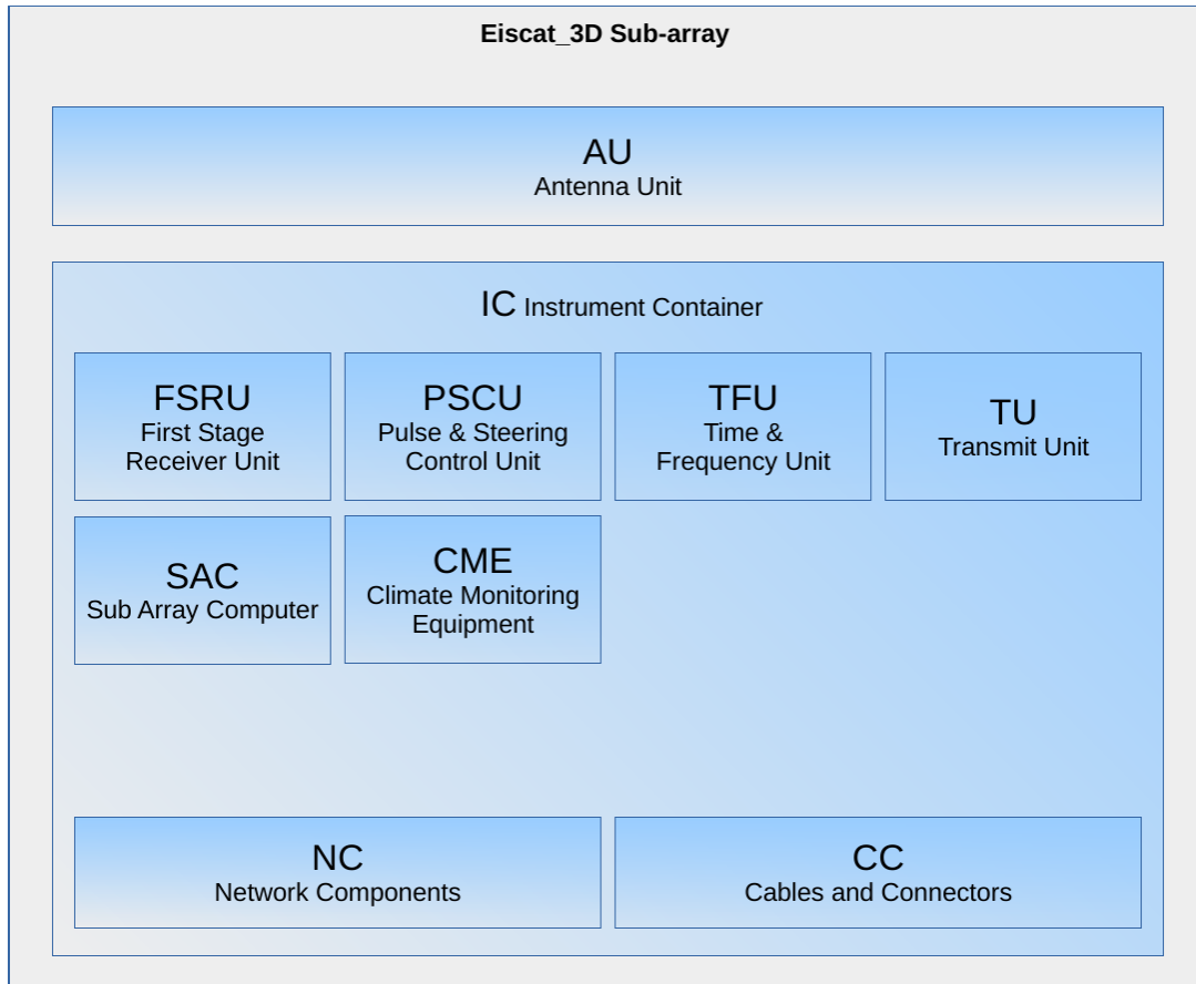
Diagram 1: The Sub-array system
