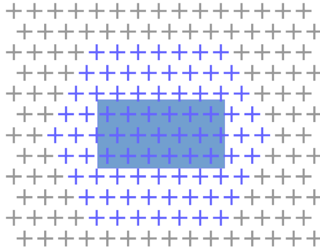
Diagram 2: EISCAT_3D Sub-array Layout
