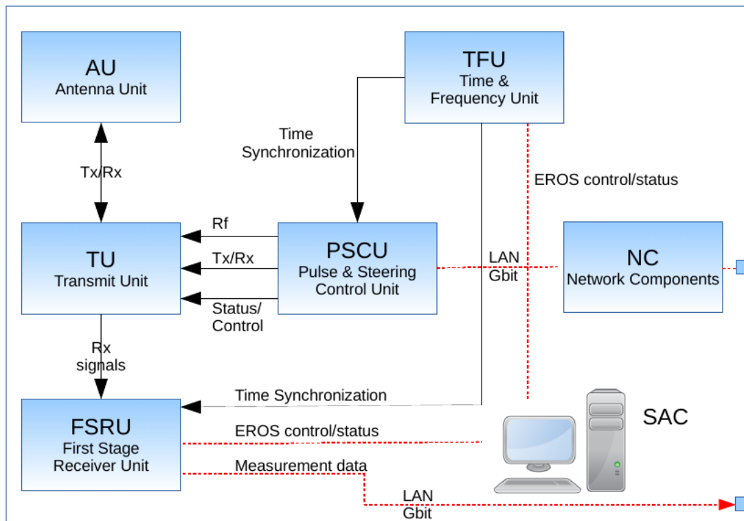
Diagram 3: Sub-array Technical systems High level Overview
