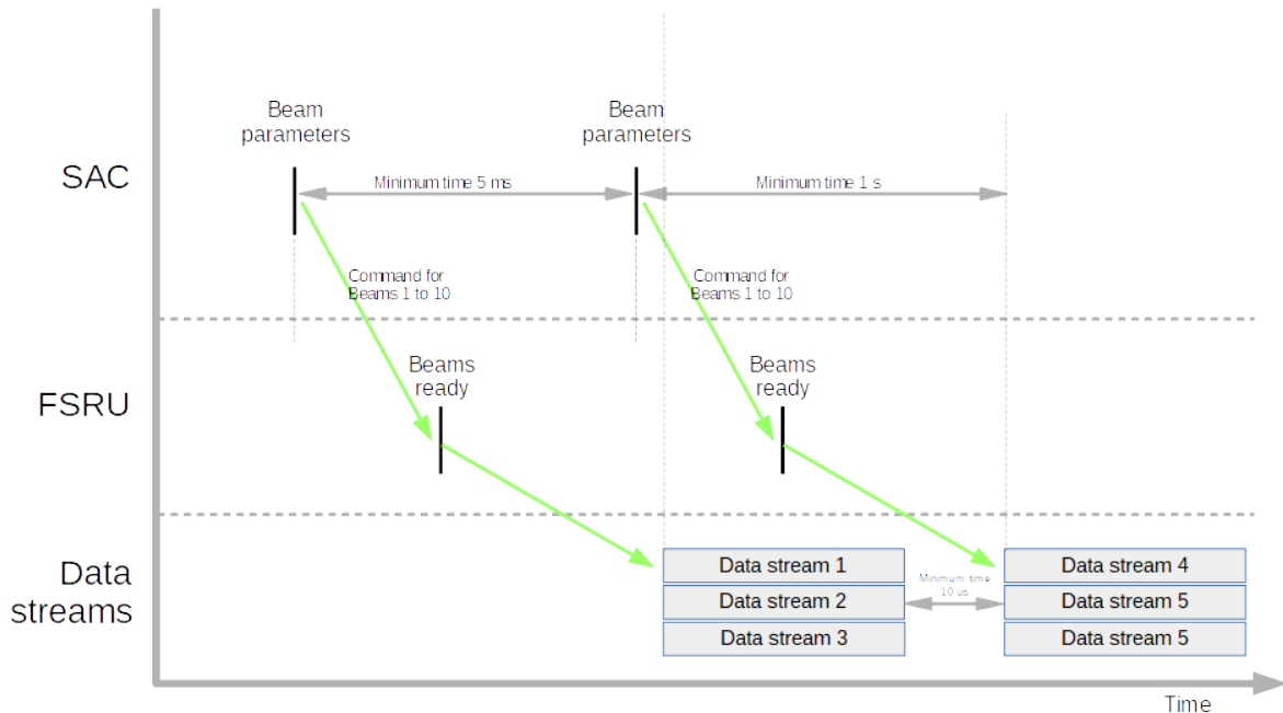
Diagram 4. Timing chart for beam parameter -command and data streams.
