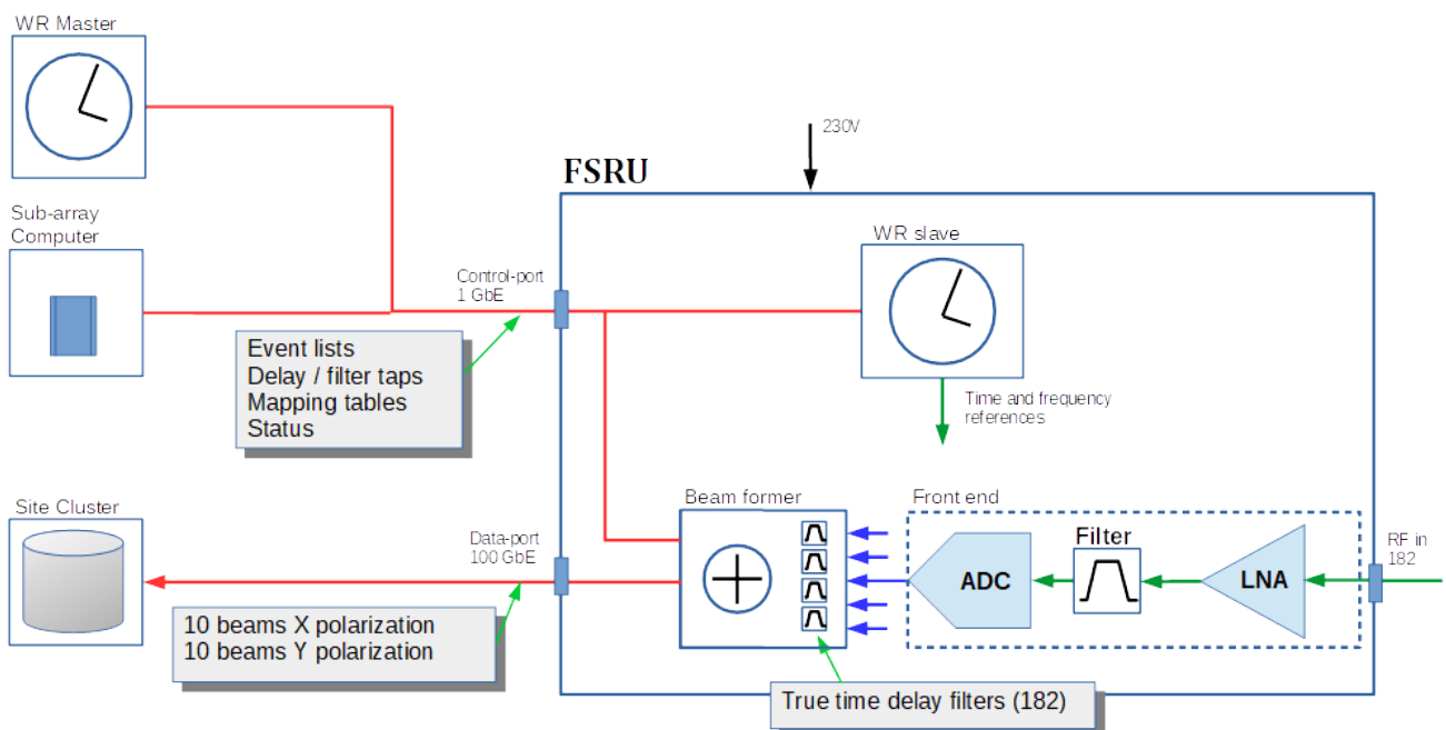
Diagram 3: First Stage Receiver Unit
