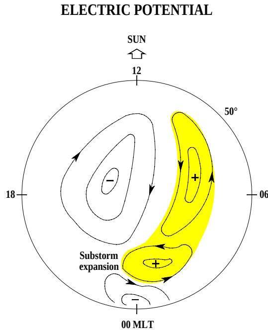
Figure 19. Schematic diagram showing two pairs of the electric potential cells, representing the effects of enhanced plasma convection and of the substorm expansion. The high potential area combining the two effects is hatched.
