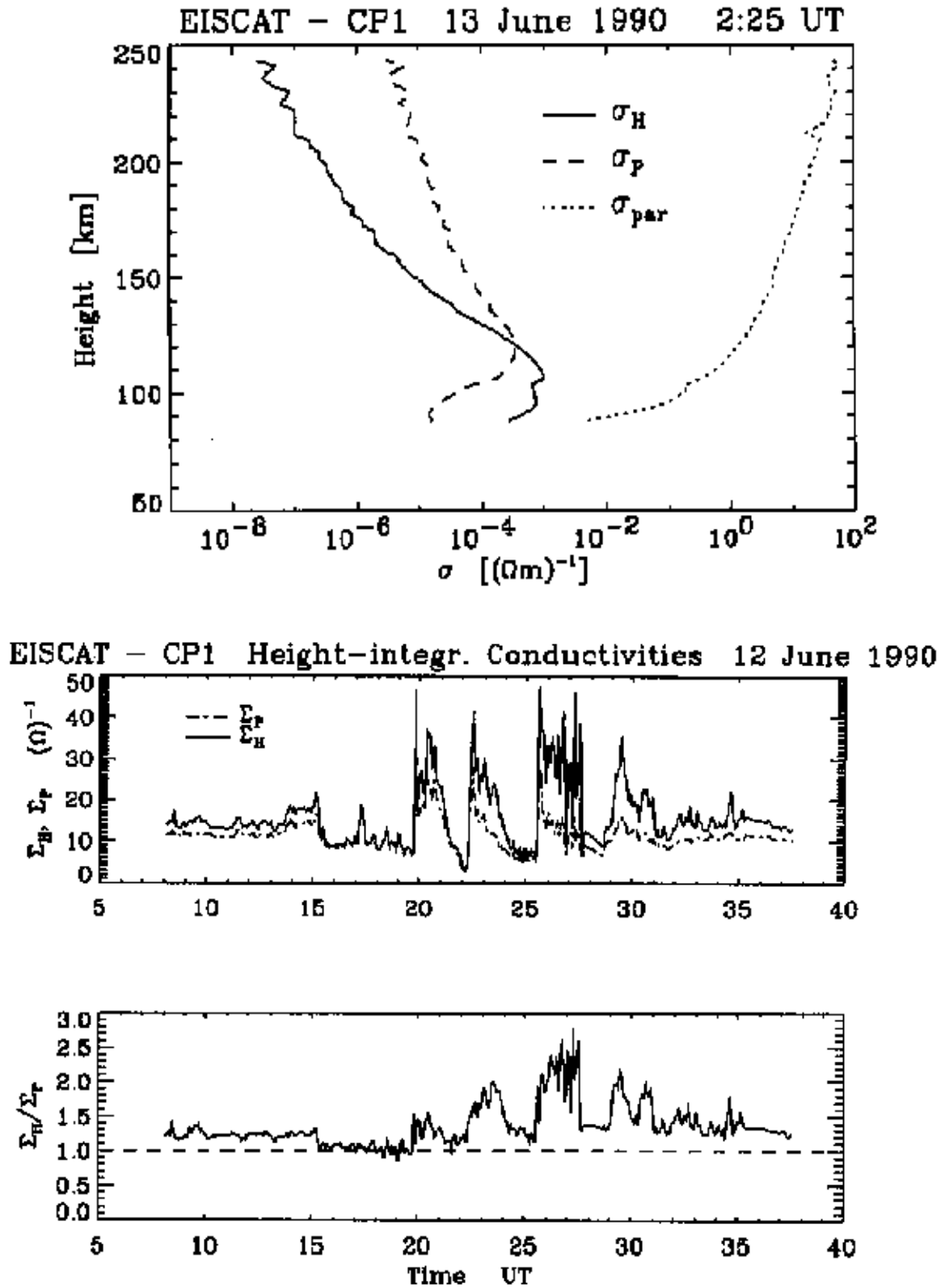
Figure 2. Upper panel: Height profiles of the components of the conductivity tensor in the ionosphere. Lower panels: Height-integrated Hall ( \Sigma_H ) and Pedersen ( \Sigma_P ) conductivities and conductivity ratio versus time.
