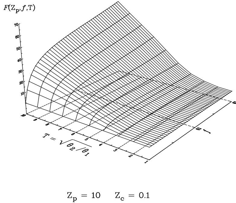
Figure 10. Plasma line enhancement factor plotted against the fraction of photoelectrons f and T = \sqrt{\theta_2/\theta_1} where \theta_2 is the temperature of the photoelectrons and \theta_1 the temperature of the background.
