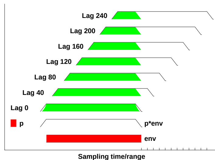
Figure 6. An illustration to show how the range ambiguity functions can be formed graphically. The pulse is 320\ \mu\text{s} long and the receiver impulse response 20\ \mu\text{s} long. The transmitter envelope env is shown at the bottom, filter impulse response p and p * env next and the range ambiguity functions at multiples of 40\ \mu\text{s} above.
