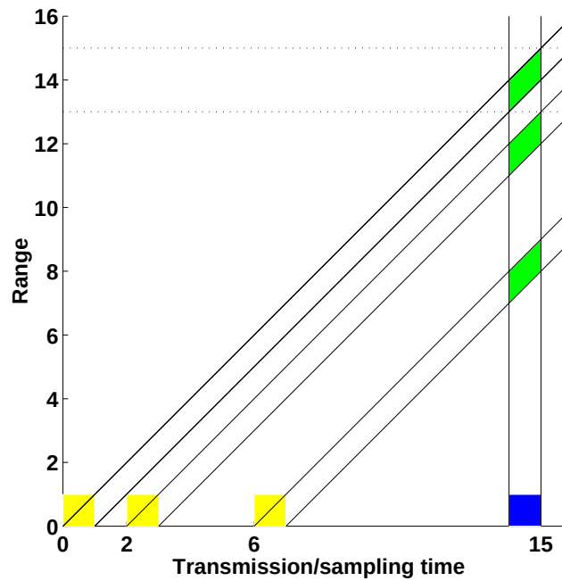
Figure 2. Range-time diagram for a three-pulse experiment. The transmitter envelope is denoted by the dotted blocks and the receiver impulse response by the solid block in the horizontal axis.
