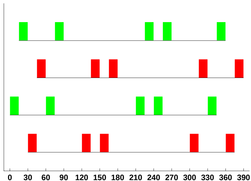
Figure 10. An interlaced 5-pulse code set used in EISCAT CP1H experiment.
