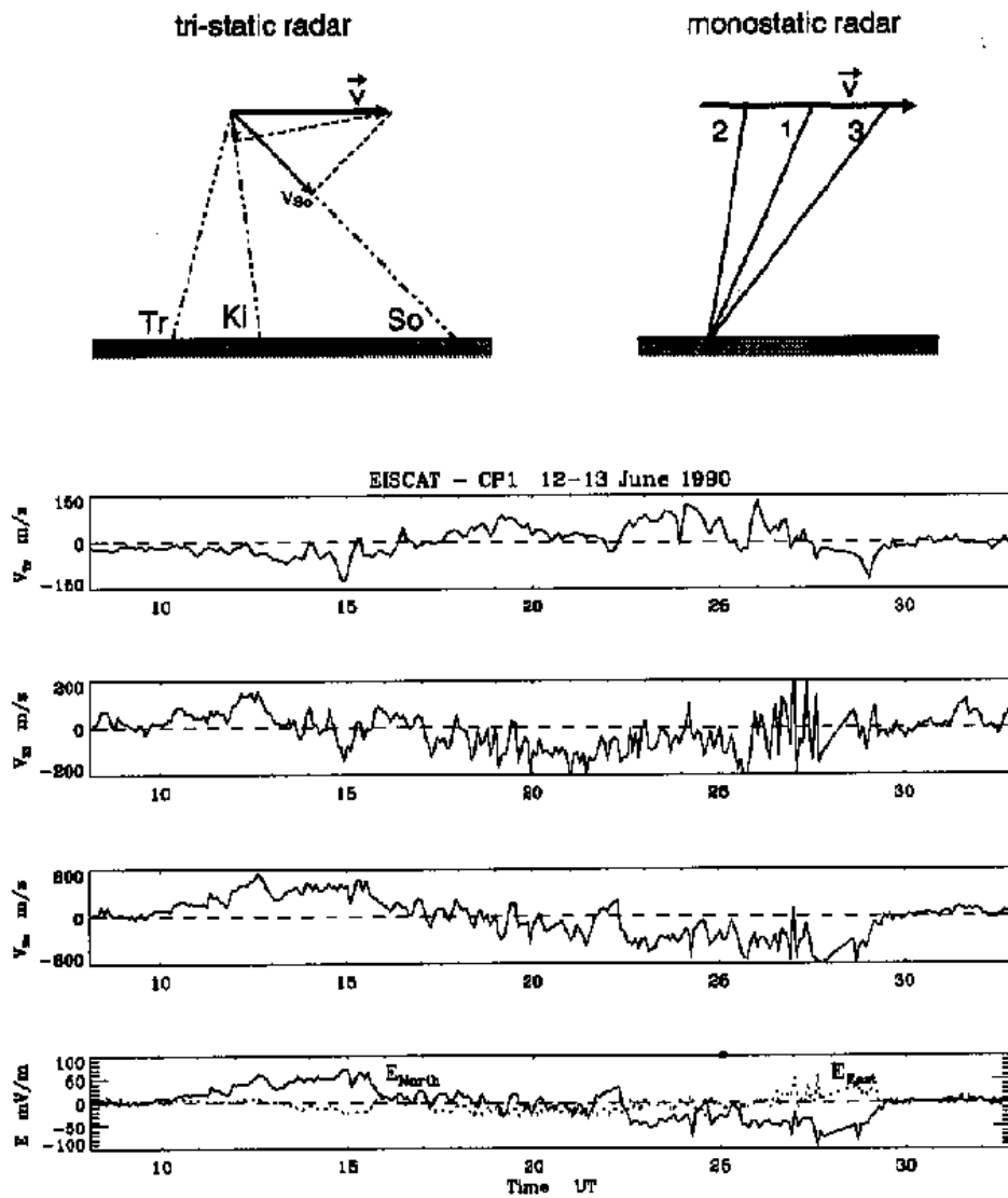
Figure 1. Measurements of the ion drift velocity vector with a tri-static(upper left) and a monostatic radar (upper right). Line-of-sight ion drift from Tromsø, Kiruna and Sodankylä and the derived electric field for a one day EISCAT experiment.
