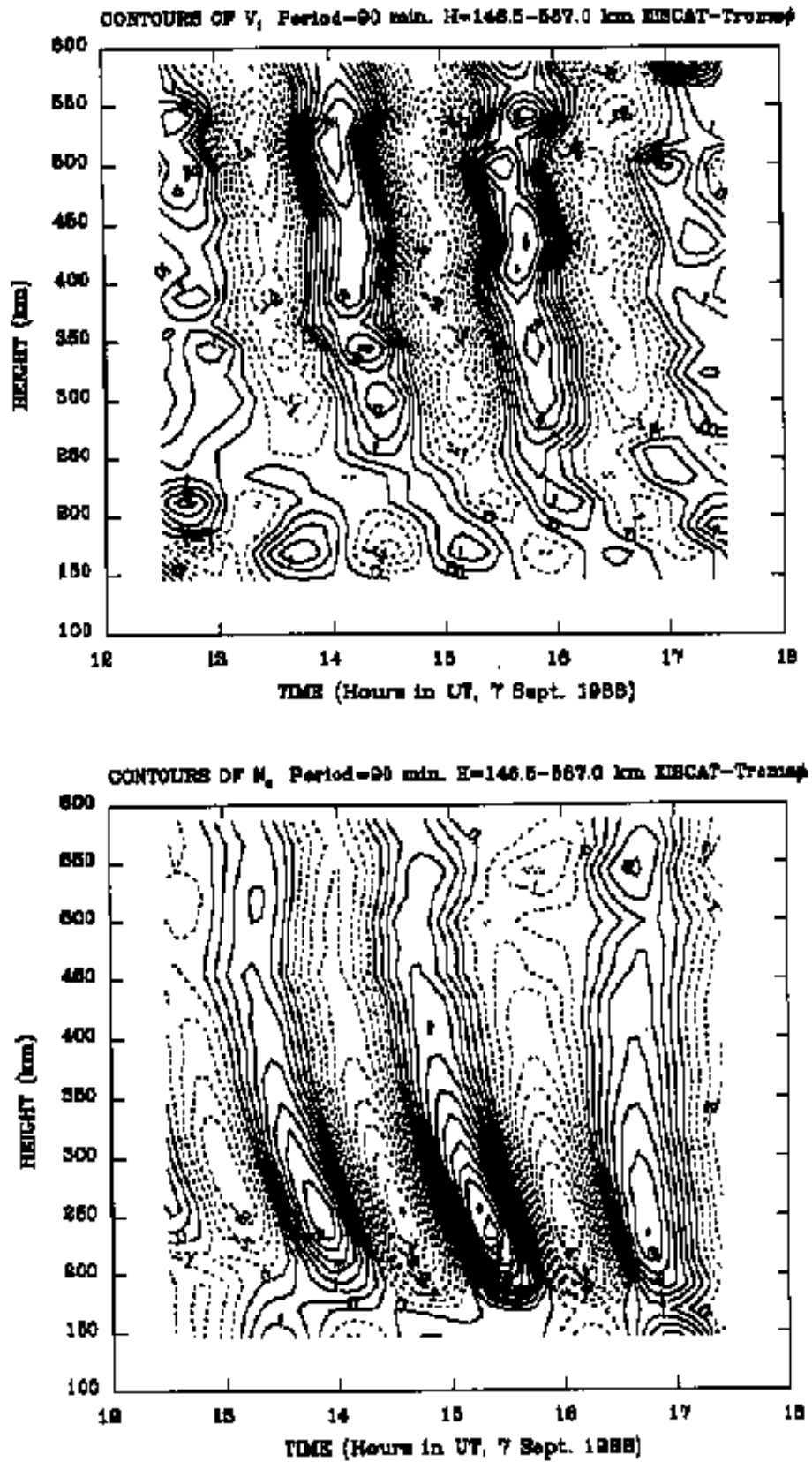
Figure 12. Waves in the line-of-sight ion drift velocity (upper panel) and in the electron density (lower panel) made visible by digital filtering of the respective time series. The bandwidth of the filter is indicated by dashed lines in Figure 11.
