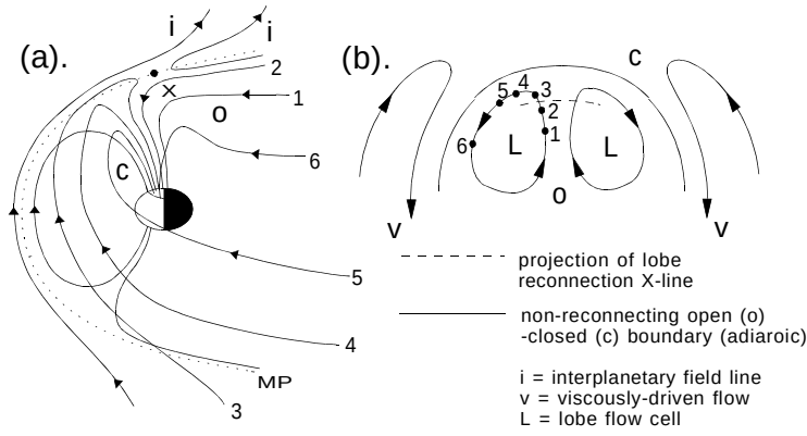
Figure 7. The same as figure 6, but for a steady-state case with reconnection at a northern-hemisphere lobe site, X , during northward IMF. In (a), the field lines 1 and 2 were opened during a prior period of southward IMF and have remained open: they are seen convecting towards X , where they are reconfigured (such that the point where they thread the magnetopause is moved from the far tail to immediately sunward of X ). Field lines 3-6 show the evolution of these reconfigured open field lines around the dusk flank of the Earth (in this case) forming a circulation in the polar cap. For the case of small B_y component of the IMF, there is a corresponding circulation on the dawn flank, and two symmetrical flow cells in the ionospheric polar cap ("lobe cells", L ) as shown in (b). These sit poleward of any viscously-driven cells, forming a four-cell pattern. In cases of large |B_y| (not shown) one of the lobe flow cells will dominate, giving a three-cell pattern with a single circulation cell in the polar cap in the sense determined by the polarity of B_y .
