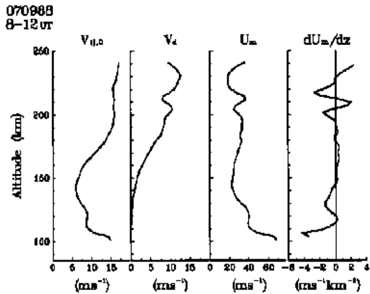
Figure 8. Height profiles of measured ion drift parallel to B ( V_{||} ), the ambipolar diffusion velocity ( V_d ), the calculated meridional neutral wind ( U_m ) and its vertical gradient.
