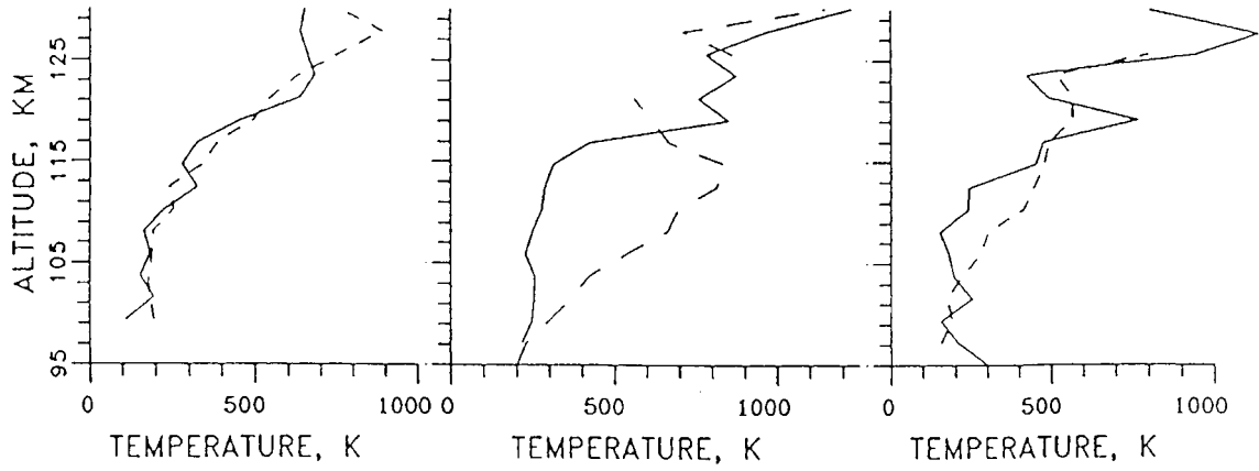
Figure 13. Ion (full lines) and electron (dashed lines) temperature profiles for selected times. There is no anomalous heating at 19.18 UT (left panel), very strong anomalous heating at 01.43 UT (centre panel), and low anomalous heating at 02.58 UT (right panel).
