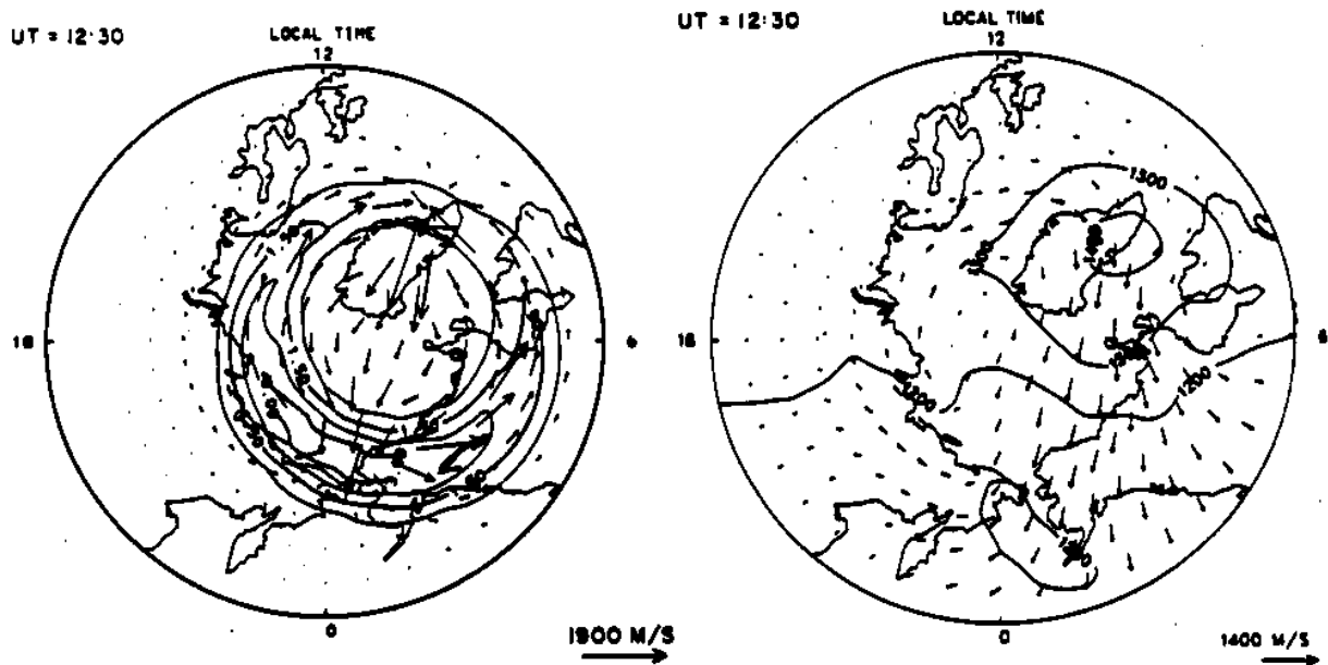
Figure 6. (Left) Horizontal component of parameterized electrodynamic drift velocities \mathbf{u}^e (arrows) and energy flux of precipitating electrons (contours with intervals of 0.75 \text{ mW} \cdot \text{m}^{-2} at 12:30 UT on 22 March 1979. (Right) Simulated neutral winds (arrows) and temperatures (contours labeled in kelvins) at approximately 300 km, at 12:30 UT on 22 March 1979. (From Roble et al., 1987).
