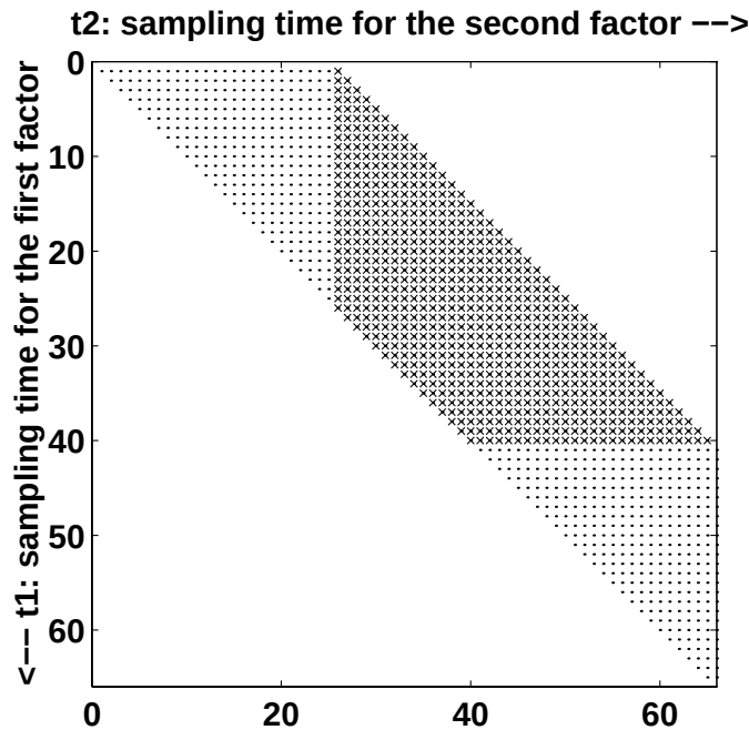
Figure 7. A lag profile matrix and crossed products belonging to a single gated long pulse measurement
