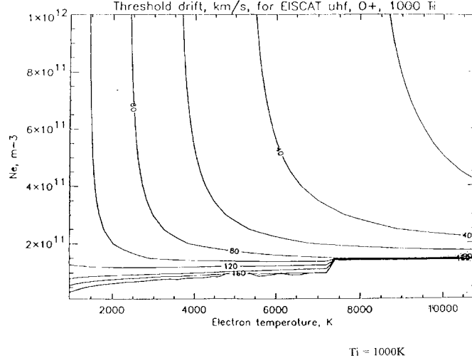
Figure 6. The threshold drift as a function of electron temperature and electron density. Ion temperature was fixed at 1000°K. For instance, for n_e = 6 \cdot 10^{11} \text{ m}^{-3} and T_e \approx 6000^\circ\text{K} , the threshold drift is 40 \text{km.s}^{-1} .
