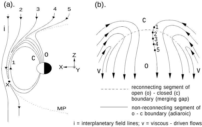
Figure 6. Schematic of the motion of newly-opened field lines away from a low-latitude reconnection site, X , when the IMF points southward. (a). Shows an noon-midnight section through the dayside magnetosphere, viewed from dusk and with the magnetopause as the dotted line MP. The field line 1 is closed (c), prior to being opened at X by reconnection with the draped interplanetary field line in the magnetosheath, i . Field lines 2-5 are open (o) field lines at different points in their subsequent evolution into the tail lobe. (b) shows the corresponding ionospheric flow streamlines in both hemispheres for steady-state conditions, the numbered dots being the locations of the field lines shown in (a): noon is at the top of the figure, dusk to the left and dawn to the right. The boundary between open and closed field lines is shown as a dashed line where it maps to the X -line (the "merging gap"), but as a solid line where it maps to a non-reconnecting segment of the magnetopause. The flows marked v are driven by viscous-like interactions between the magnetosheath flow and closed field lines.
