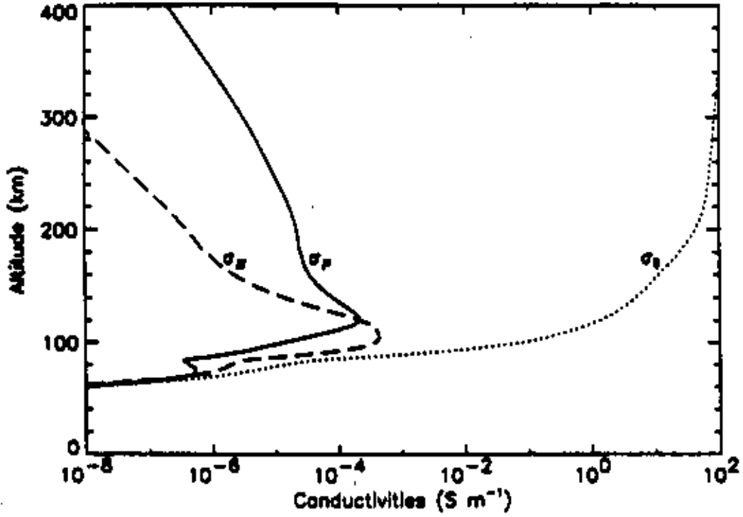
Figure 5. Noontime parallel ( \sigma_{//} ), Pedersen ( \sigma_P ), and Hall ( \sigma_H ) conductivities at 44.6°N, 2.2°E, for solar-minimum conditions on March 21. (From Richmond, 1995b).
