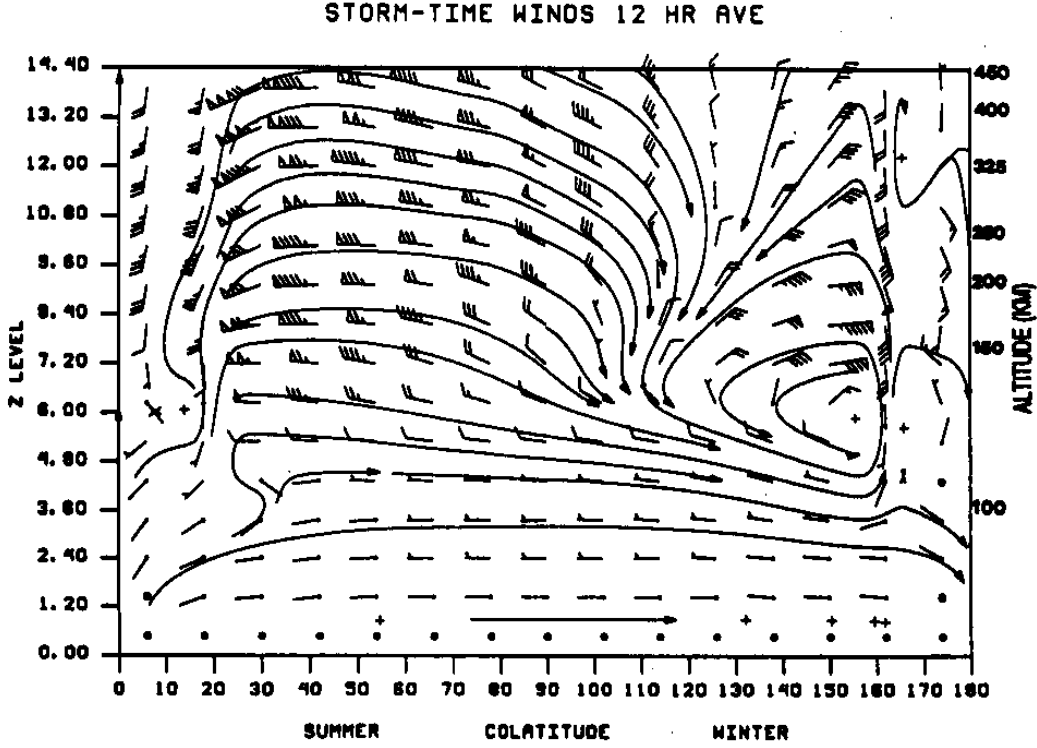
Figure 8. Meridional wind and streamlines between 80 km and 450 km averaged over 12 hours of a simulated storm at solstice using a two-dimensional model. The Z level is defined by a value of p_0 = 1.05 Pa in (10). The wind-barb notation is as follows: short barb ( 5 \text{ m.s}^{-1} ); long barb ( 10 \text{ m.s}^{-1} ); and flag ( 50 \text{ m.s}^{-1} ). The vertical components of the winds have been scaled so that the shafts of the wind arrows are parallel to streamlines. The normal summer-to winter flow is altered by Joule heating that is centered around 21^\circ and 159^\circ colatitude. The summertime equatorward flow is strengthened, while the normal wintertime poleward flow is reversed at middle latitudes. (From Brinkman et al., 1992).
