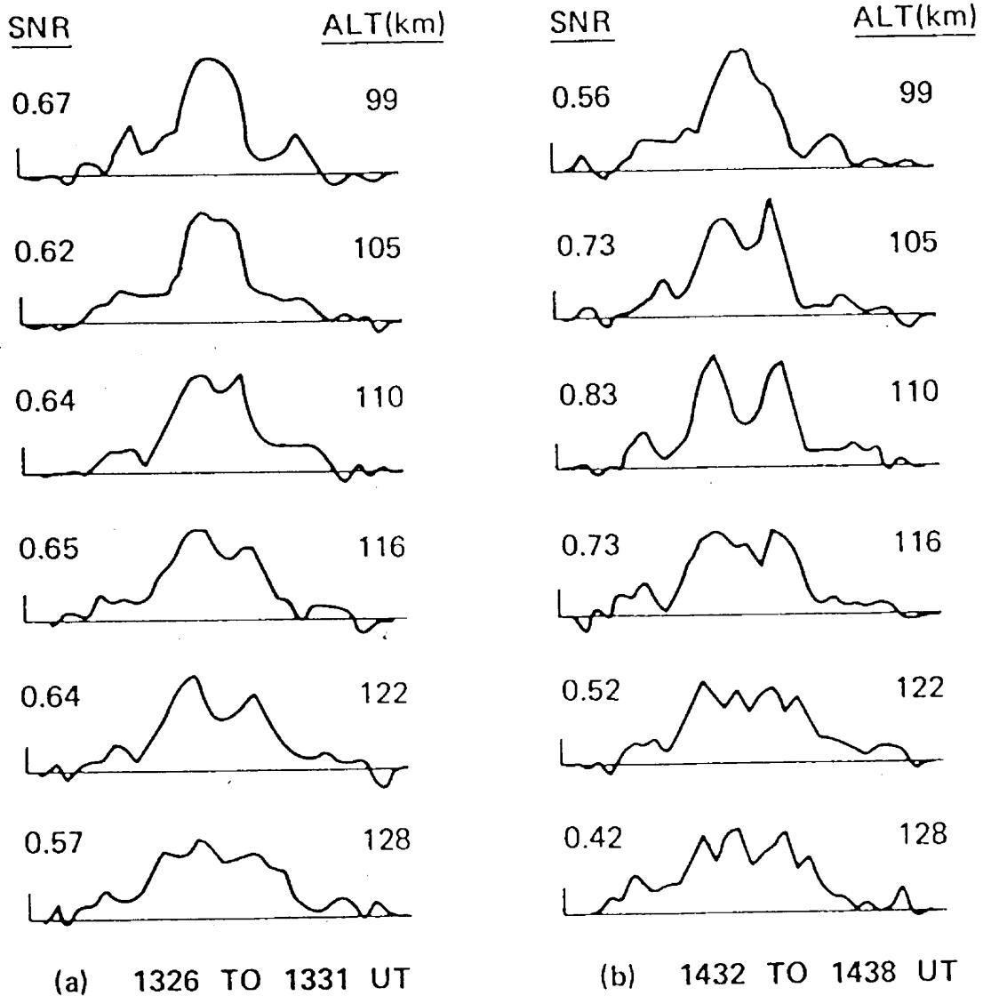
Figure 12. E region spectra from March 18, 1978, obtained with the multipulse autocorrelator using a 60- \mu s unipulse followed one interpulse period later by a burst of three 60- \mu s pulses that started at 0, 100 and 340 \mu s. The spectral window is 50 kHz wide. The two time periods were selected, in part, because of similar signal-to-noise ratios. (a) Typical spectra measured between 1326 and 1331 UT. (b) Unusual spectra measured between 1432 and 1438 UT. In particular, they are unusual at 105 and 110 km, though at 116 km the spectrum is still considerably wider than that in the earlier time period.
