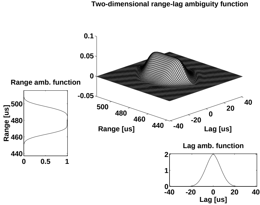
Figure 4. Two-dimensional and reduced ambiguity functions for the 40 \mu s pulse of EISCAT CP1K-experiment
